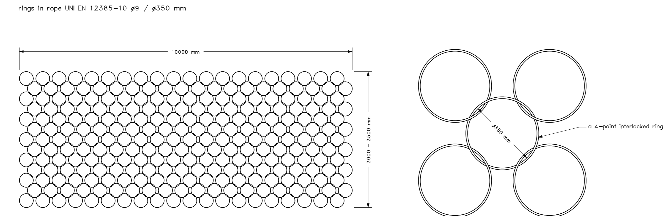
DETAIL OF RING PANEL
