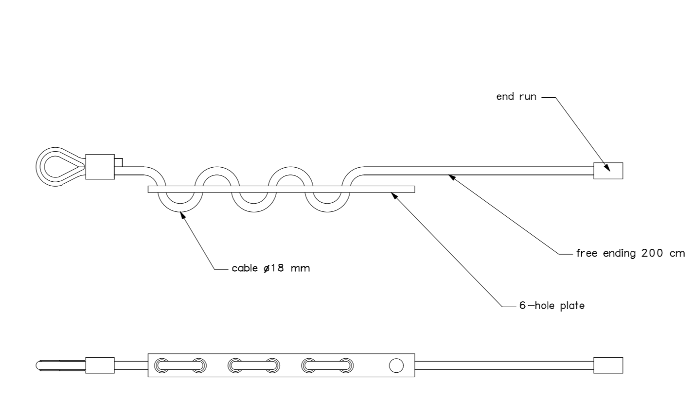
BRAKE SYSTEM #18 mm / 200 kJ
