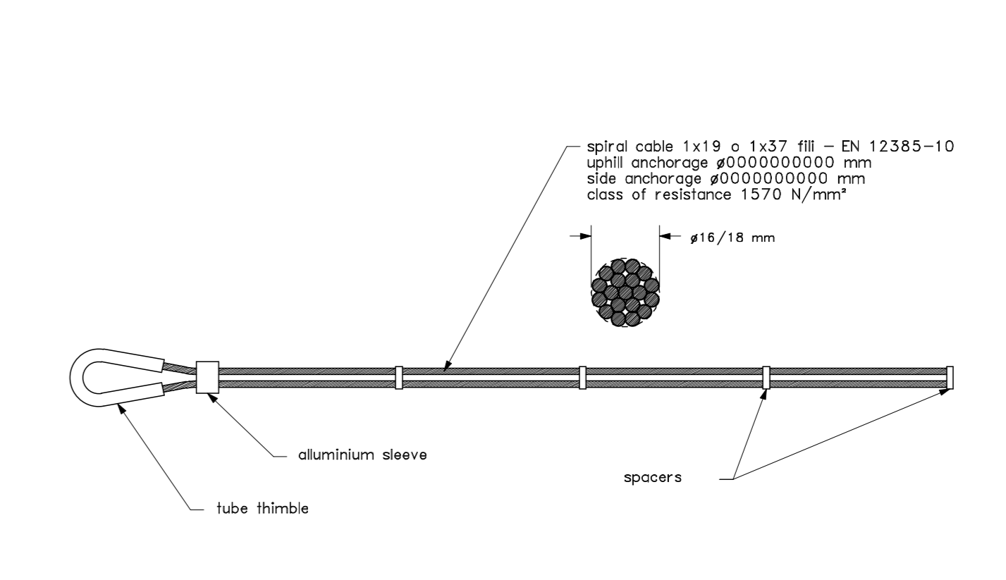
SPIRAL CABLE ANCHOR upper #0000000000 mm / side #0000000000 mm
