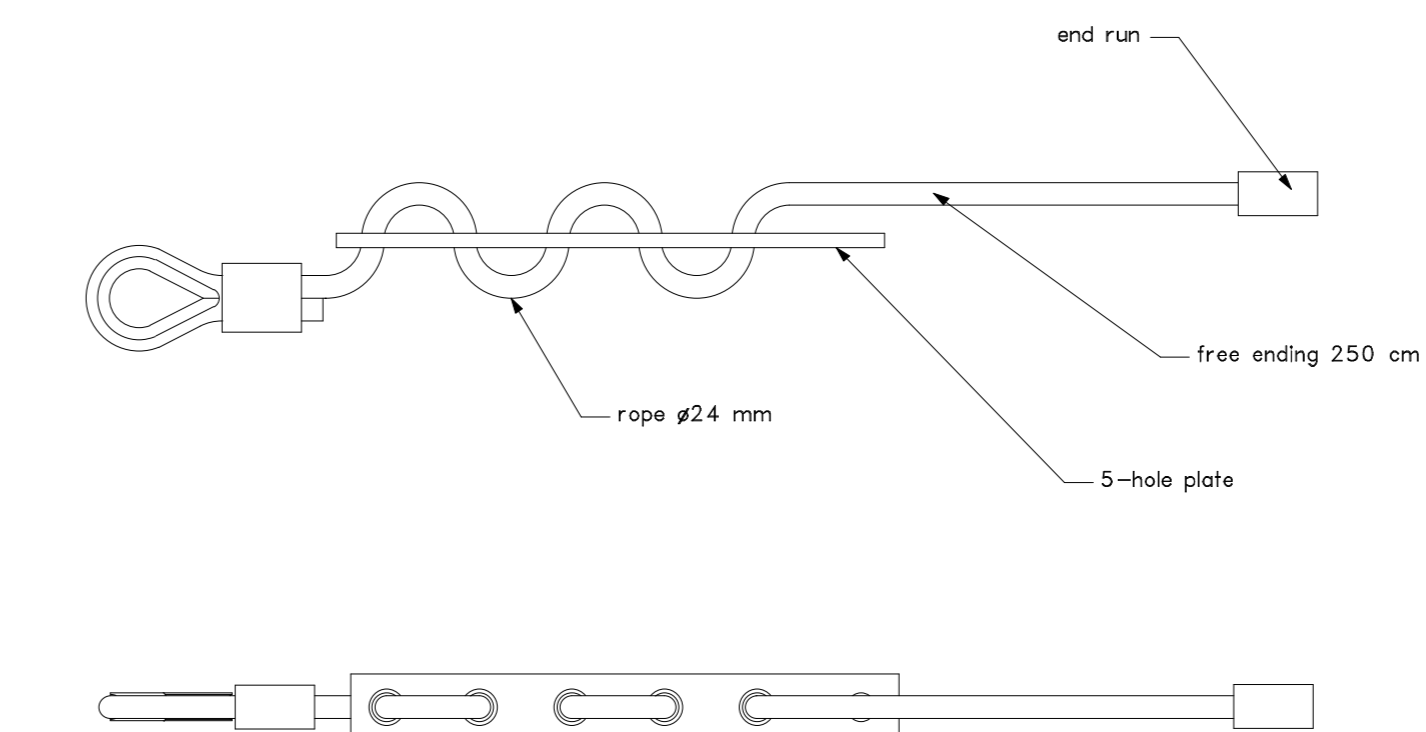
BRAKE SYSTEM #24 mm / 250 kJ
