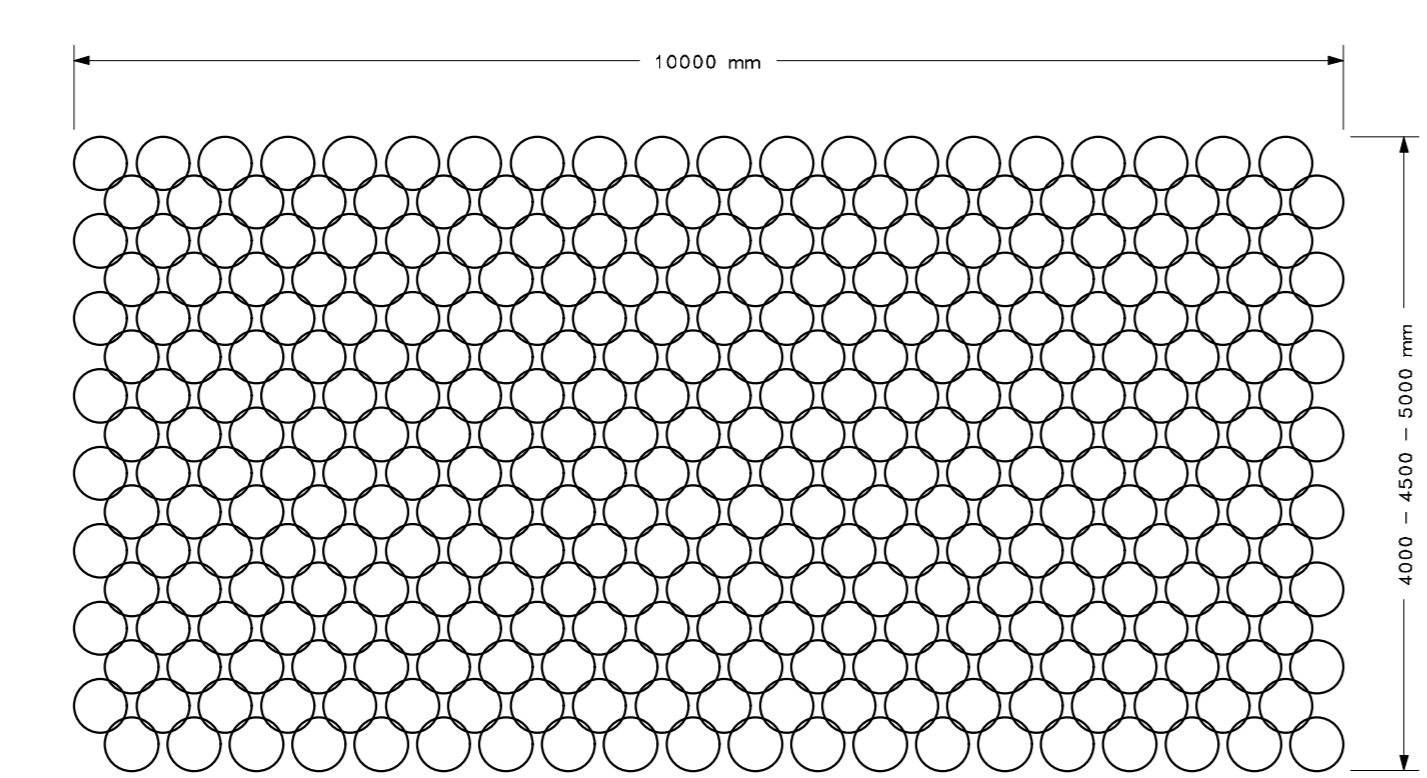
DETAIL OF RING PANEL rings in rope UNI EN 12385-10 #10, 5 / #350 mm
