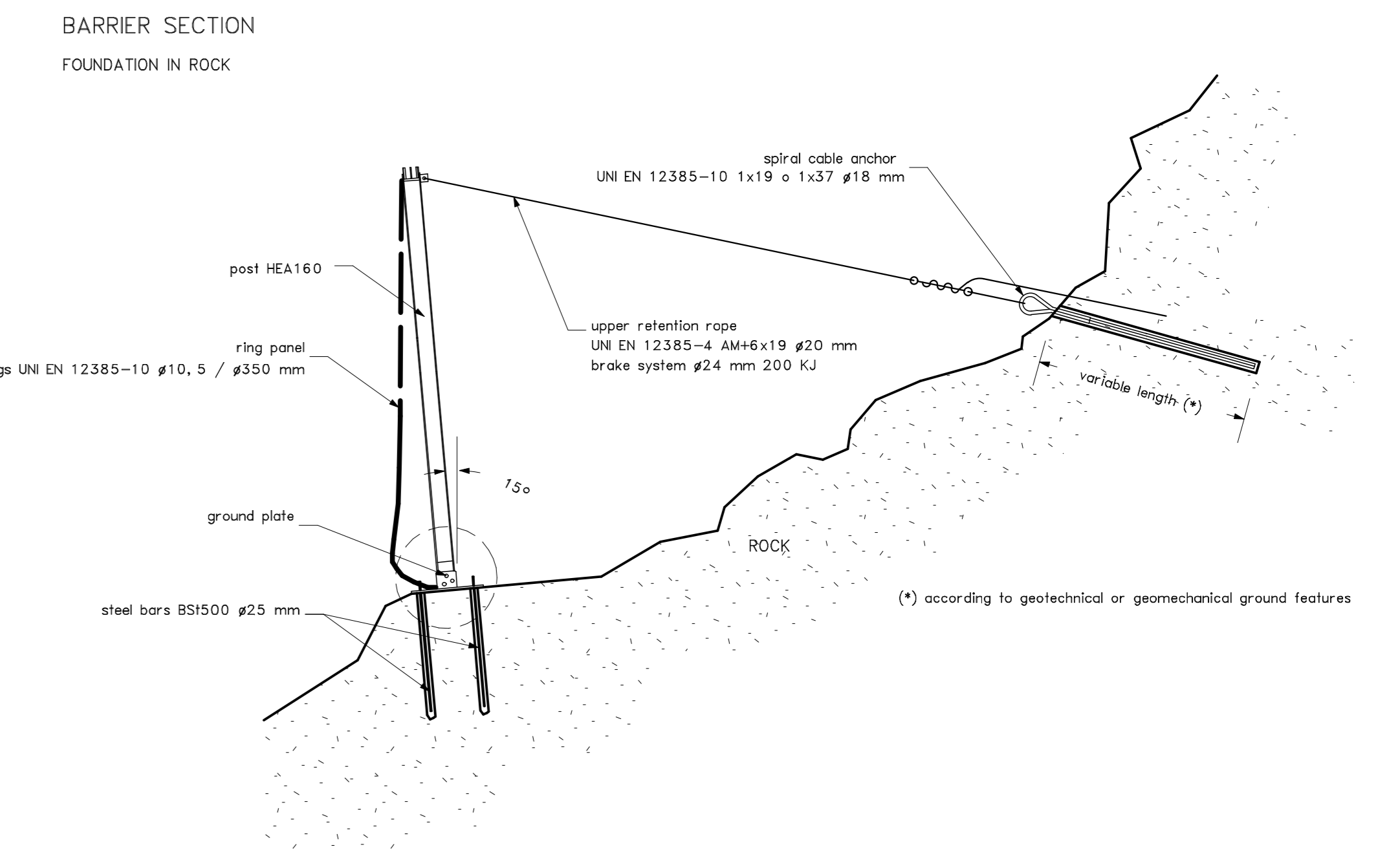
SPIRAL CABLE ANCHOR upper #18 mm / side #18 mm
