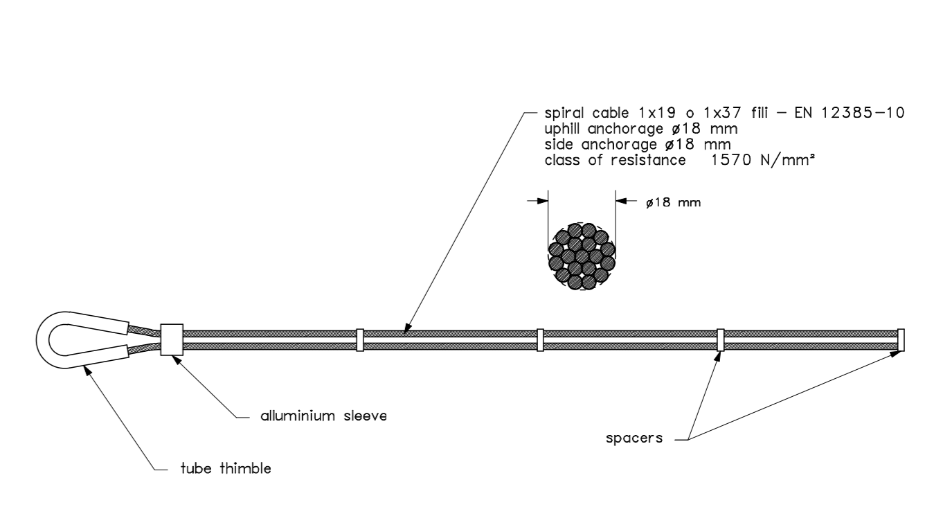
SPIRAL CABLE ANCHOR upper #18 mm / side #18 mm
